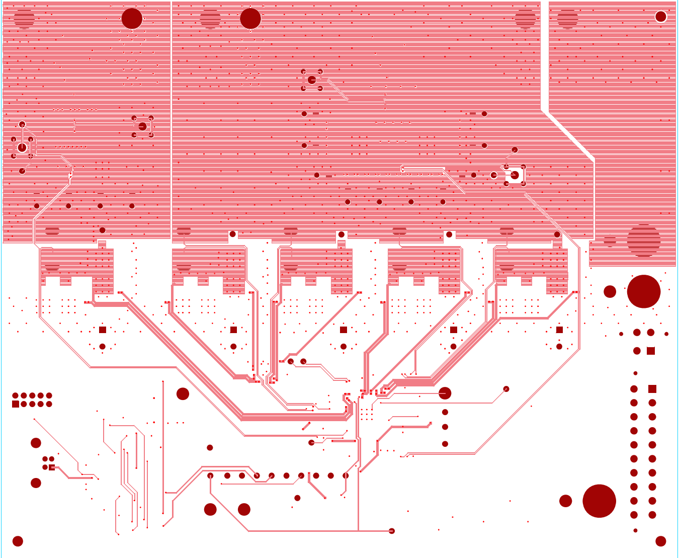
FIGURE 24. BOTTOM
